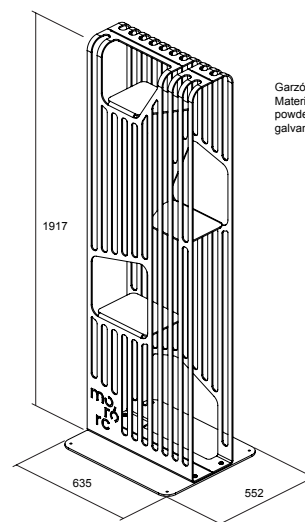
Garzón O Materials: powder coated aluminum galvanised & powdercoated steel
