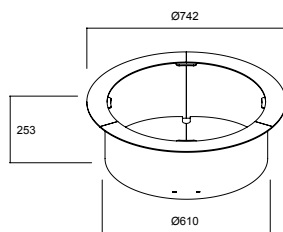
ROCCO / fire basket materials: weathering steel
