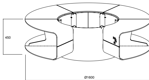
ROCCO / base materials: powder coated aluminum zinc coated adjustable feet
